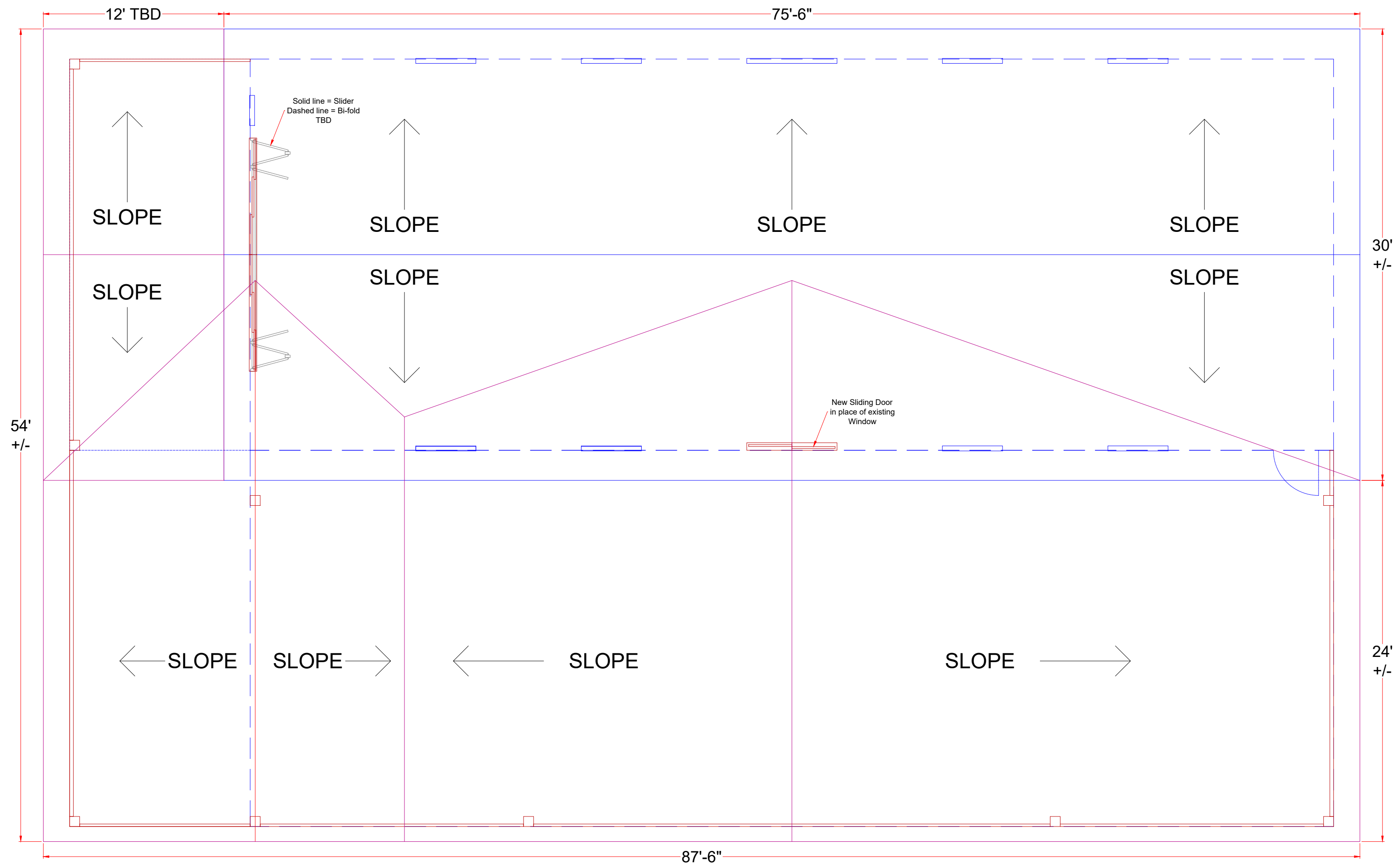
OVERHEAD VIEW / ROOF AND DECK - SECTION SECOND STORY AND ABOVE
