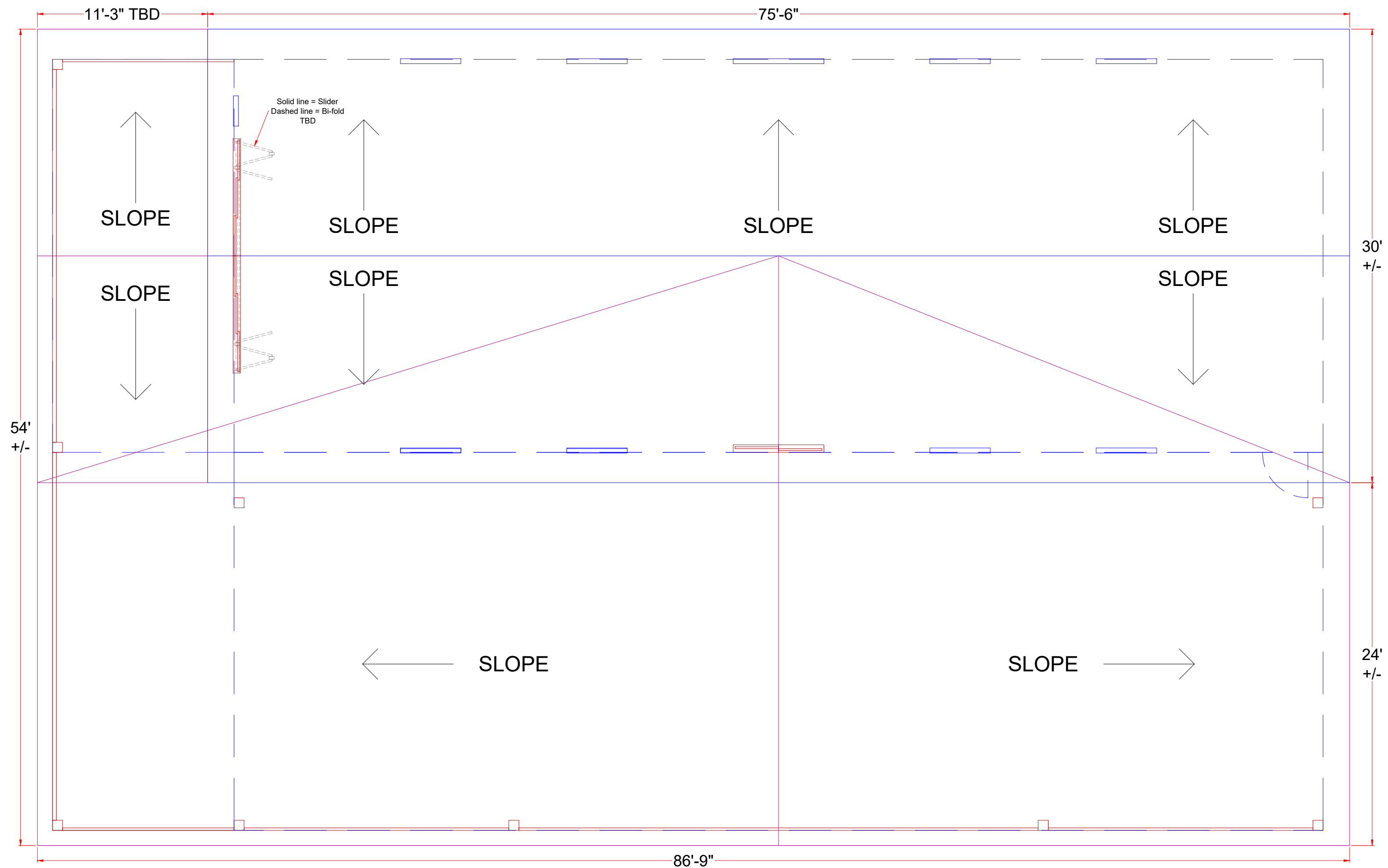
OVERHEAD VIEW / ROOF AND DECK - SECTION SECOND STORY AND ABOVE
